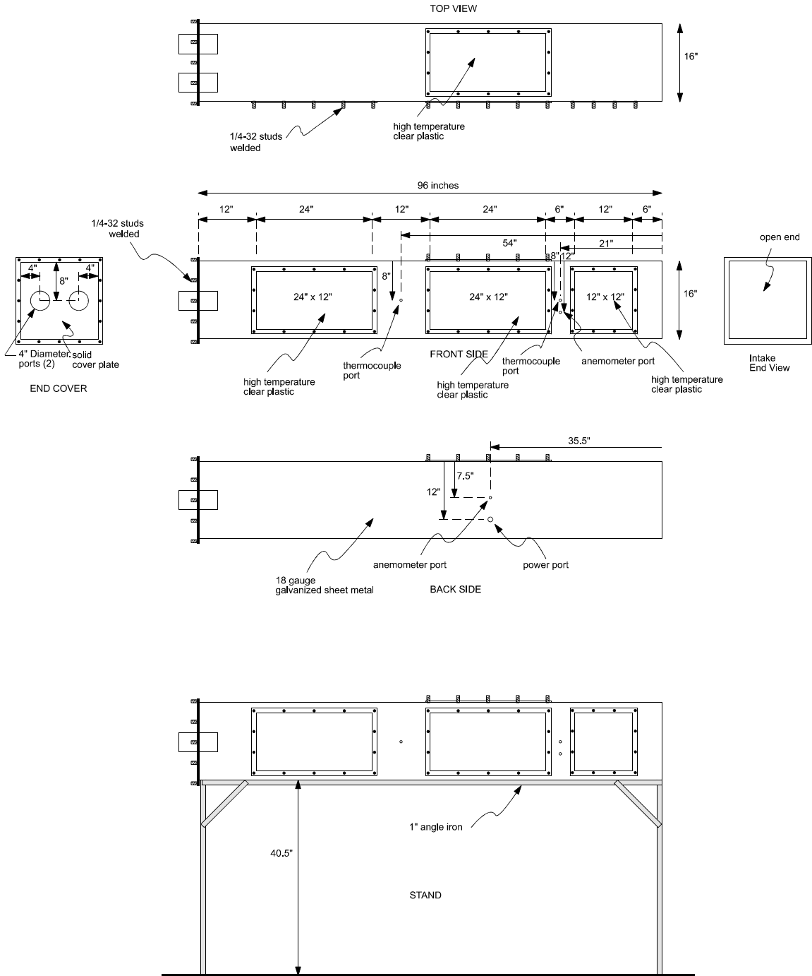
Figure H-1a. Dimensions of Test Setup Box
