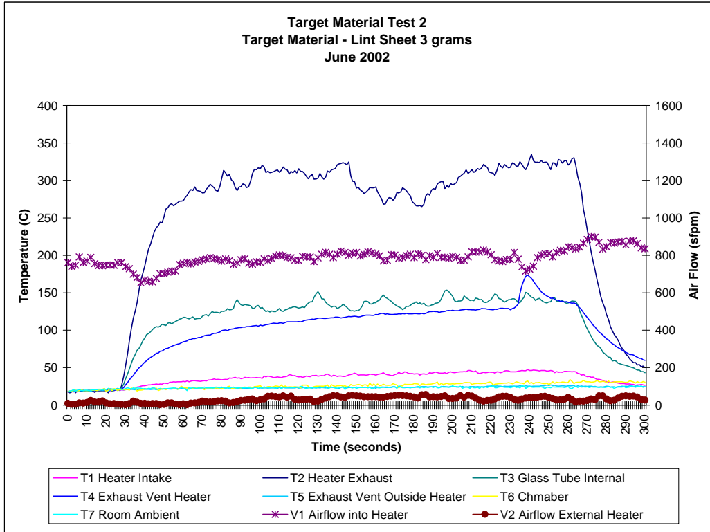
Figure H-2. Target Material Test 2 Data
