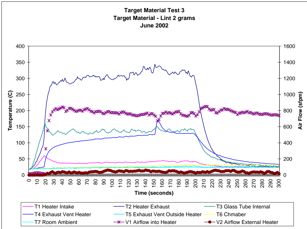
Figure H-3. Target Material Test 3 Data
