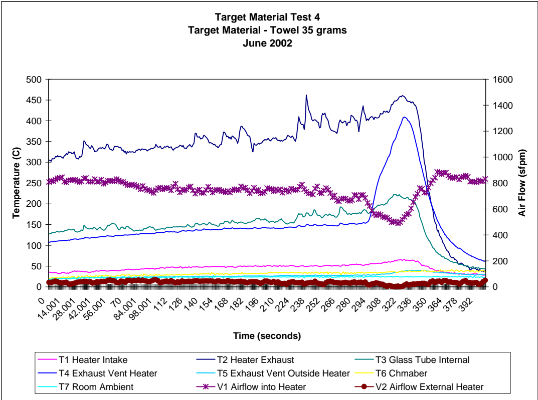
Figure H-4. Target Material Test 4 Data
