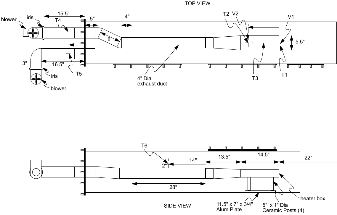
Figure H-1b. Dimensions of Heater Setup
