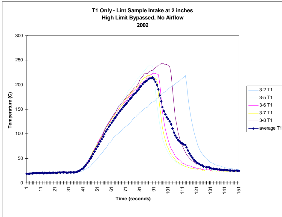
Figure I-5. T1 Only – 2 Inches from the Heater Housing Edge
