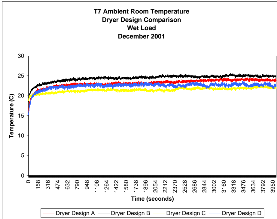
Figure I-3. T7 Ambient Temperature Dryer Design Comparison
