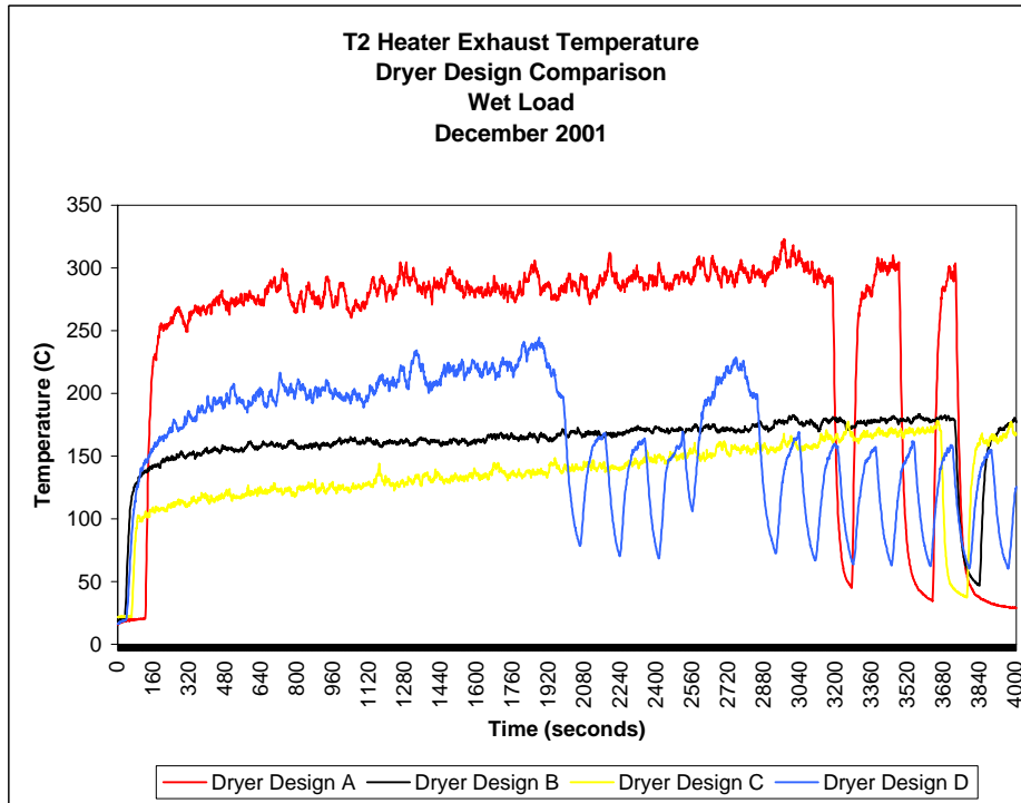
Figure I-1. T2 Heater Exhaust Dryer Design Comparison
