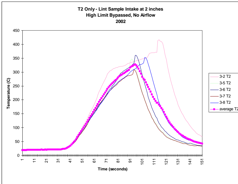
Figure I-6. T2 Only – 2 Inches from the Heater Housing Edge
