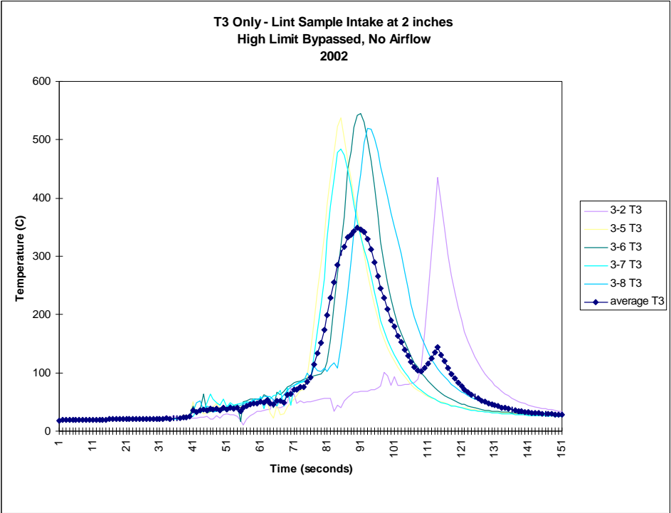
Figure I-7. T3 Only – 2 Inches from the Heater Housing Edge
