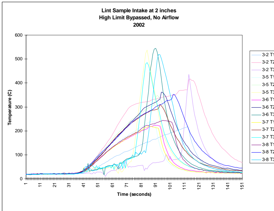
Figure I-4. Lint Samples tested 2 Inches from Heater Edge
